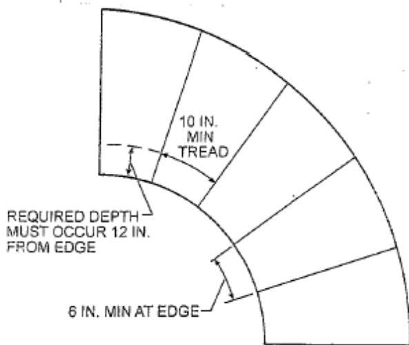
Figure R311.5.3.2(2) WINDERS USED FOR CIRCULAR STAIRWAY
