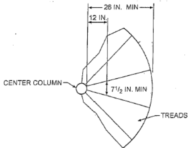
Figure R311.5.8.1 SPIRAL STAIRS
