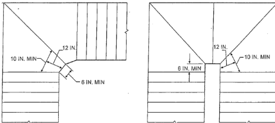
Figure R311.5.3.2(1) WINDERS
