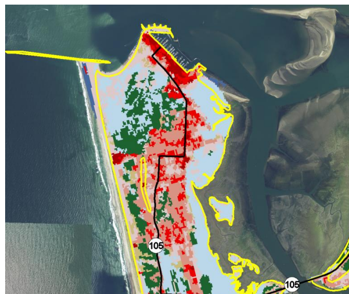
Figure 2. Aerial view of West Port. The solid yellow line marks the tsunami hazard zone. Colored areas show intensity of development (based on land cover data).
